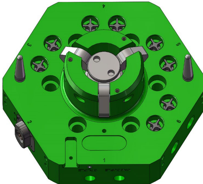
Figure 8.1.2.1-1. E80 Robot Side Visual Inspection
