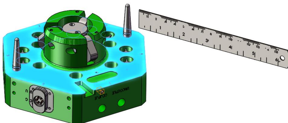
Figure 8.1.3-1. Robot Side – Raised Material Inspection
