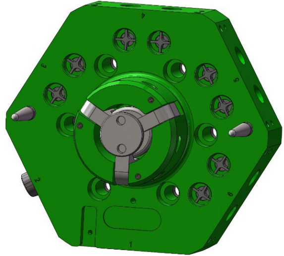
Figure 6.1-2. Robot Side Uncoupled (Cams Retracted)
