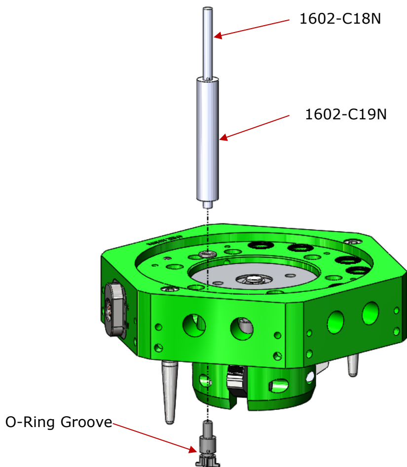
Figure 10.1.3-2. Poppet Valve Installation
