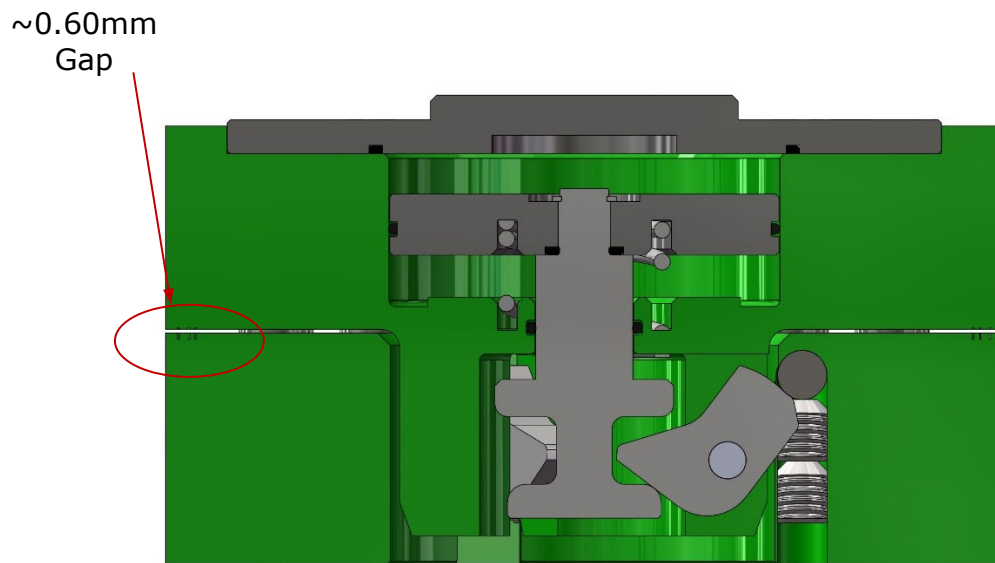
Figure 6.3.1-2. E80 Robot & Tool Side – Loss of Air Mechanical Lock
