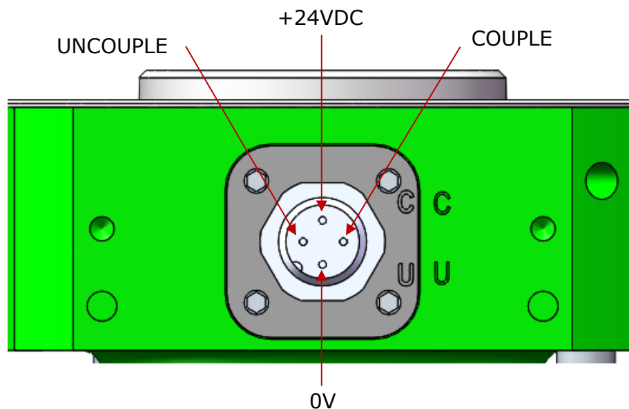
Figure 5.4-2. M12 Couple/Uncouple Signal Interface
