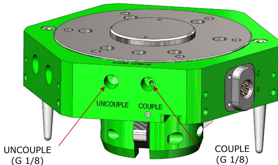
Figure 5.3-1. E80 Robot Side Air Supply Ports
