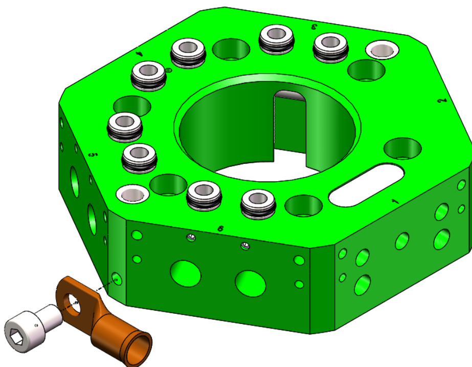
Figure 5.7-3. Grounding M6 Lug Mounting
