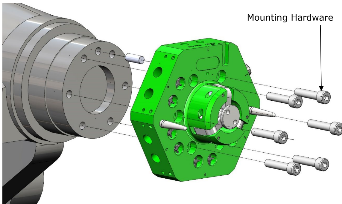
Figure 5.1.1-1. E80 Robot Side Installation w/ M8 Hardware
