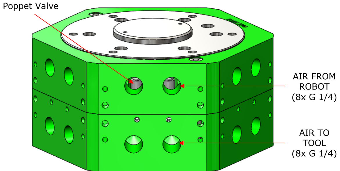
Figure 5.6-1. E80 User Pneumatic Ports
