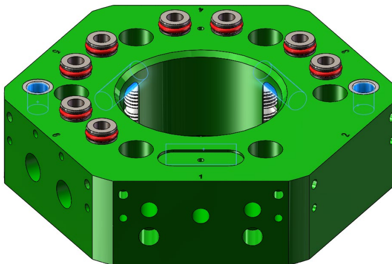
Figure 8.1.1.1-1. ET100 Tool Side Lubrication
