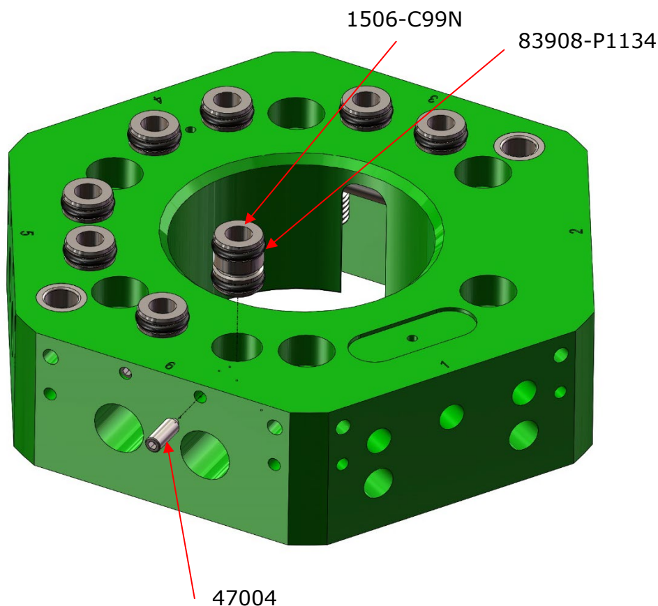
Figure 10.2.2-1. Air Valve Fitting Replacement
