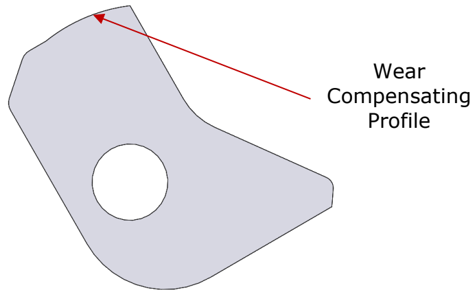
Figure 6.3.1-1. E80 Cam Mechanical Lock Feature
