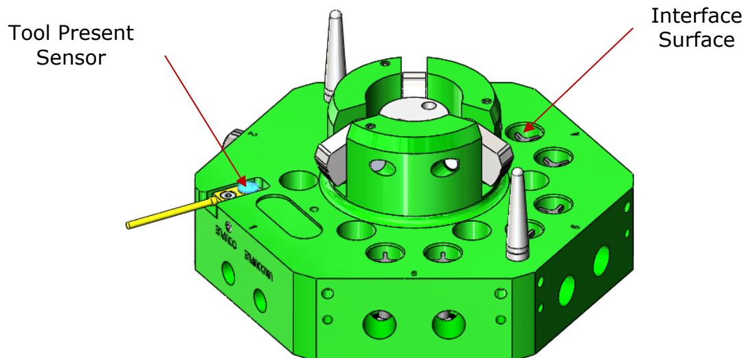
Figure 5.5-2. Tool Present Sensor Installation
