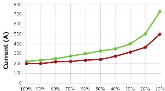
Current vs Duty Cycle, at 20 °C (68 °F) and 0-1000 Hz
