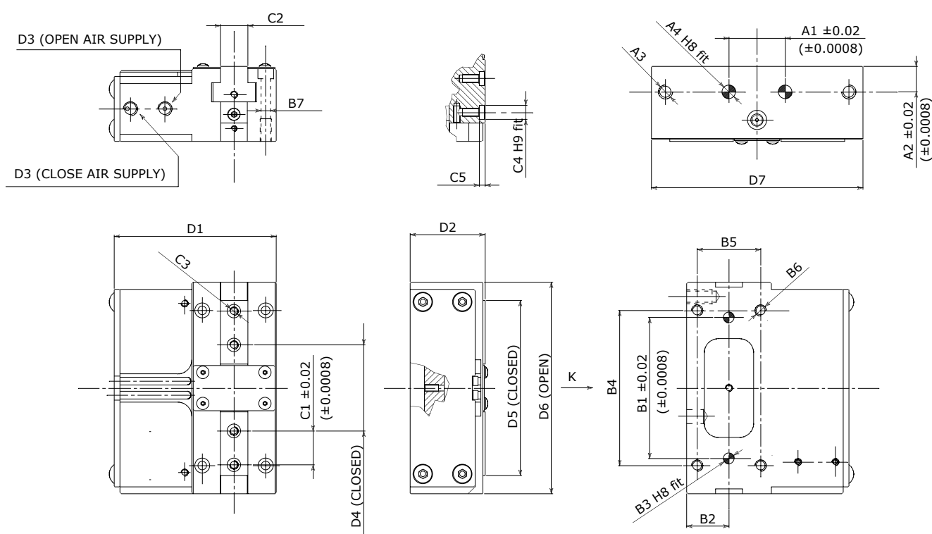
VIEW "K"
