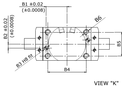
VIEW "K"
