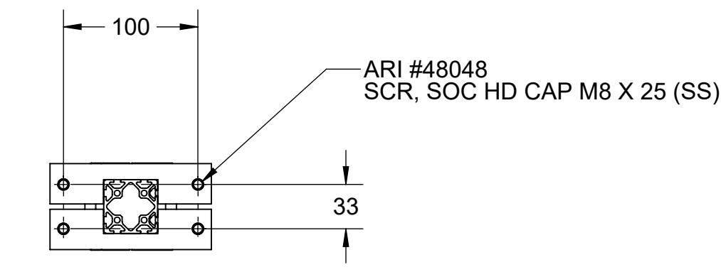
MOUNTING PATTERN
