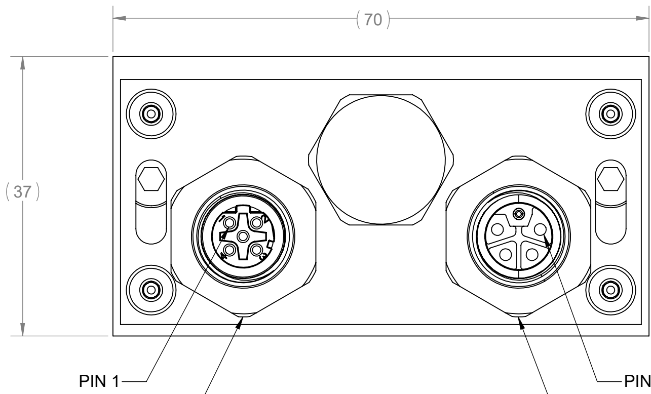
CONNECTOR, 4 SOC, M12 D-CODED, M16 X 1.5 CONNECTOR, 5 SOC, M12 L-CODED, M16 X 1.5
