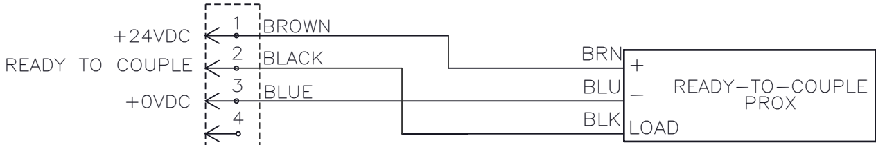
ARI #1307-P66N 4 PIN M12 CONNECTOR
