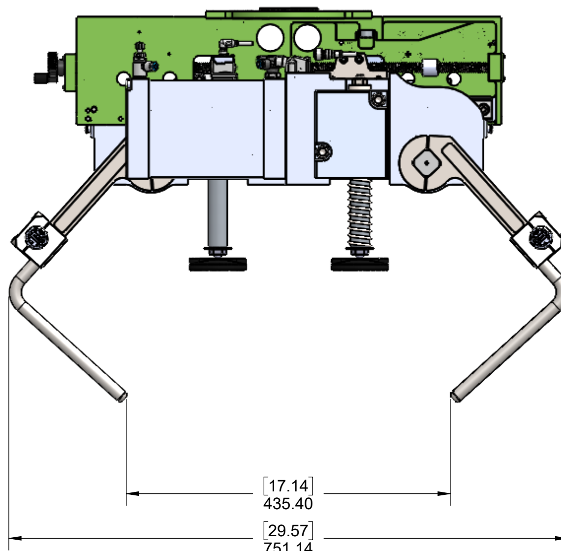
GRIPPER MINIMUM WIDTH FINGERS OPEN
