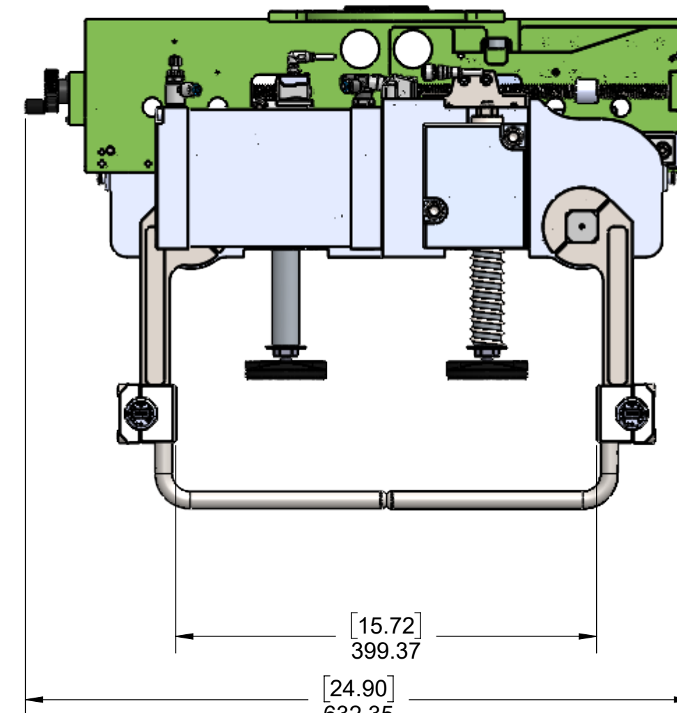
GRIPPER MINIMUM WIDTH FINGERS CLOSED
