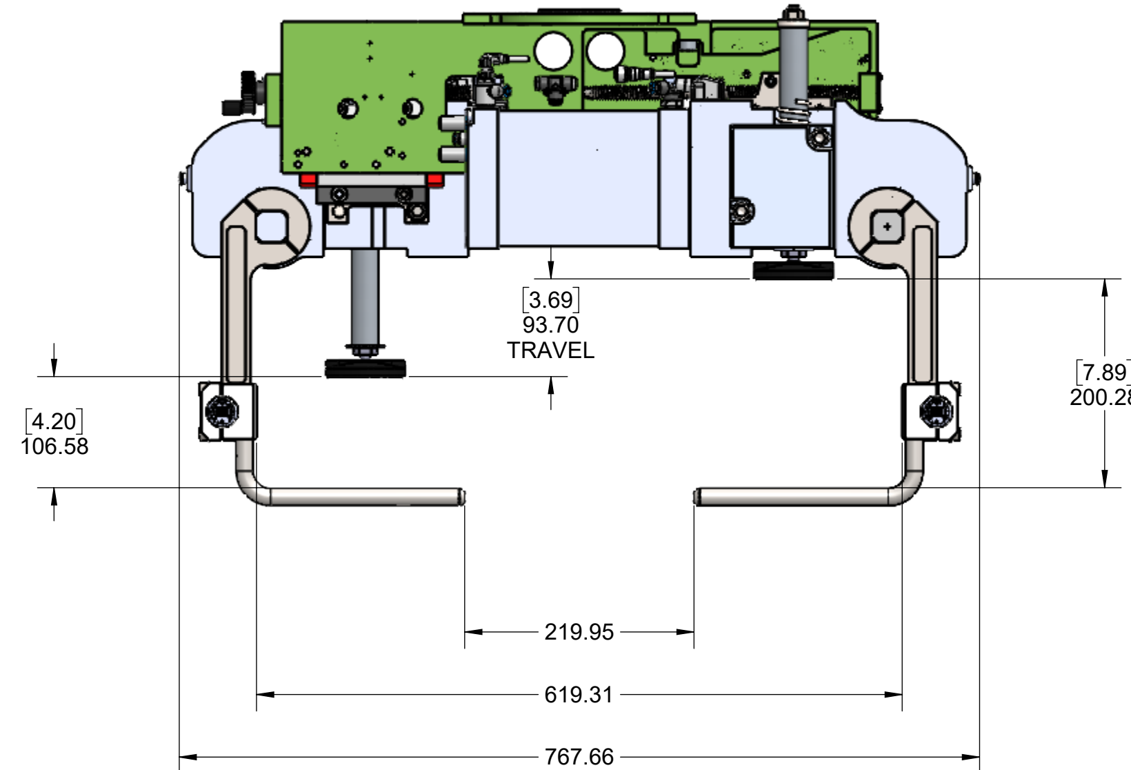
GRIPPER MAXINIUM WIDTH FINGERS CLOSED
