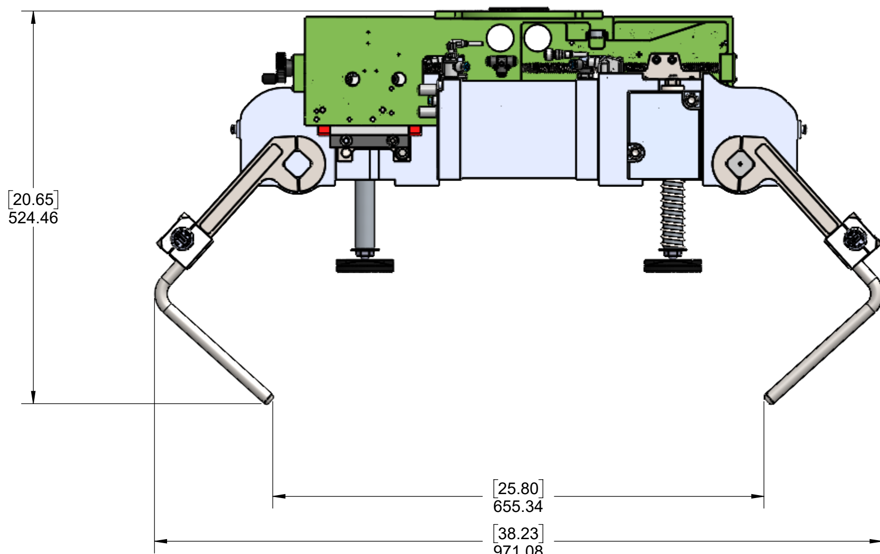
GRIPPER MAXINIUM WIDTH FINGERS OPEN
