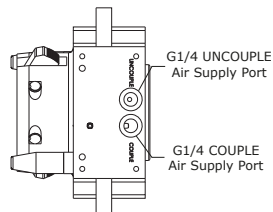
VIEW B-B
